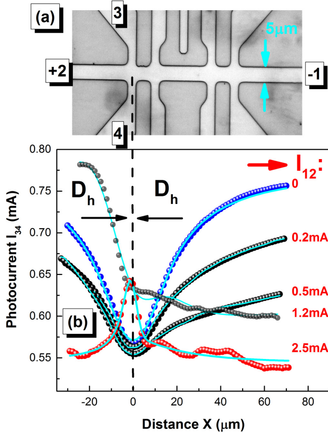
FIG. 2. (a) Microscope image of the sample. (b) Photocurrent I_{34} (circles) measured at T = 3.7 K between collecting probes 3 and 4 at different electric currents I_{12} through probes 1 and 2. The cyan lines represent calculated spatial diffusion profiles. Black and red arrows indicate the directions of hole diffusion and electric current, respectively.
