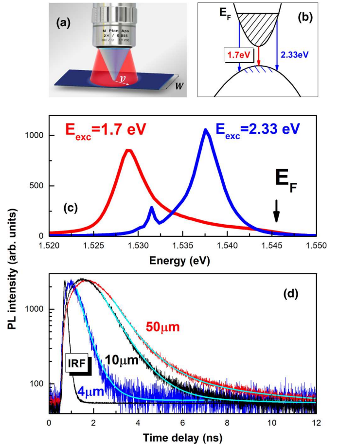
FIG. 1. (a) Sketch of the excitation/collection probe, (b) scheme of PL transitions at different laser excitation energies, (c) typical PL spectra measured at T = 4 K and laser excitation at 440 nm (2.33 eV) and 730 nm (1.7 eV) at a pump power of 7.5 \mu\text{W} , and (d) typical PL decay transients measured in channel sections of different widths 4, 10, and 50 \mu\text{m} at T = 4 K and laser excitation at 440 nm (2.33 eV); the cyan lines show the results of the best fits.
